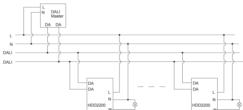
Wiring Diagram
